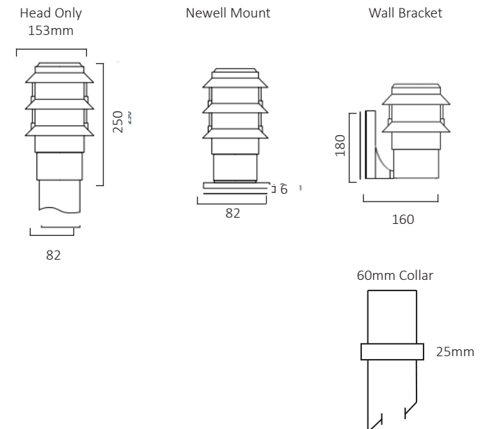
** Images showing 82mm post fitting
